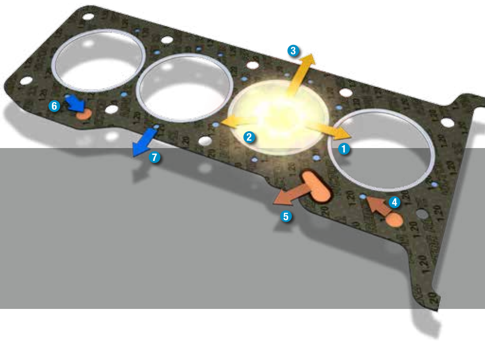
◀ Typical media leakages with composite cylinder-head gaskets.
